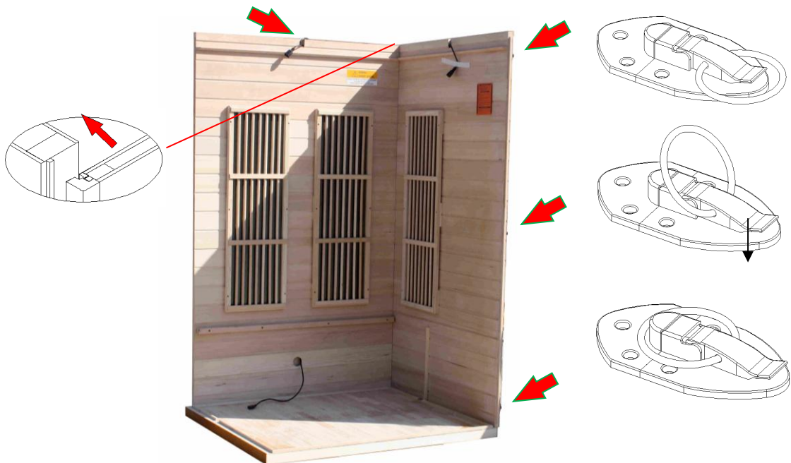
FIG 5 Assembling Left Side Panel
