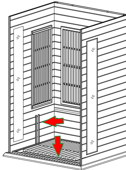
FIG 8 Placing Floor Heater
