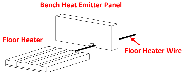
FIG 8.1 Connect Floor Heater
