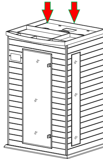
FIG 14 Installing Roof Cover
