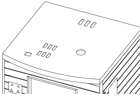
FIG 7 Slip the power cord through Roof Cover (Roof Cover is optional to install)
