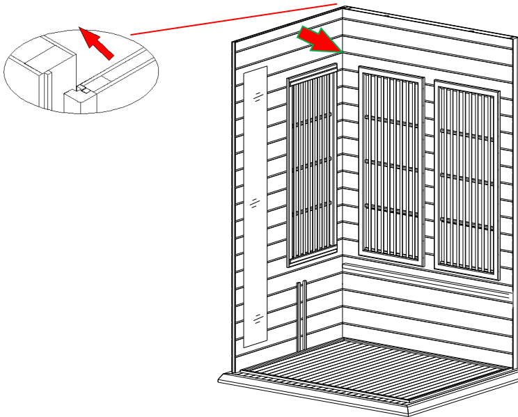
FIG-4 Assembling Left Side Panel
