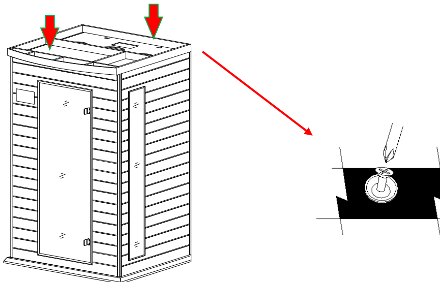
FIG-14 Screwing down ROOF PANEL
