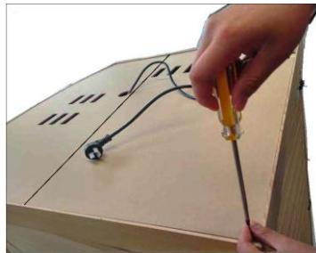
FIG-17 Roof Dust Cover Assembly (optional to install)
