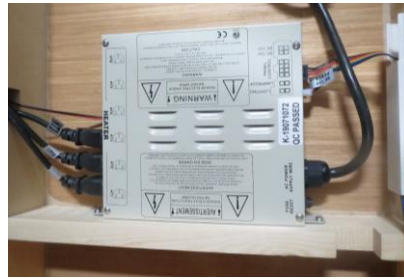
Figure 1 (2) Power Supplies
