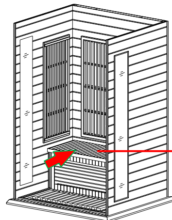
FIG 10 Installing Bench
