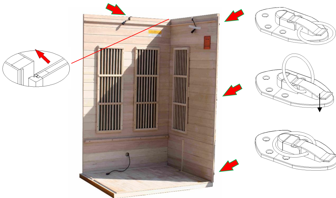
FIG 5 Assembling Right Side Panel
