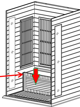
FIG 9 Installing Bench Heat Emitter
