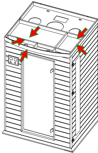
FIG 12 Slip cords/wires through corresponding holes
