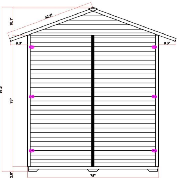
Rear Panel Outside View
