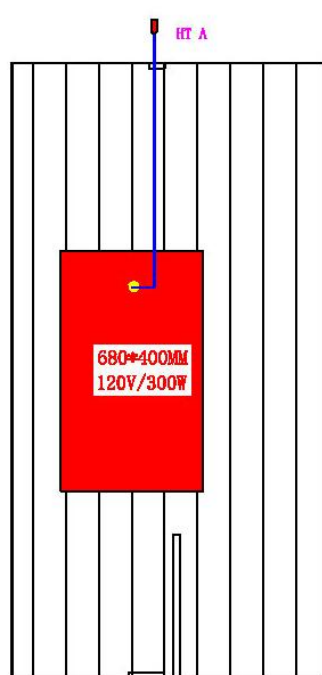
Right side wall panel
