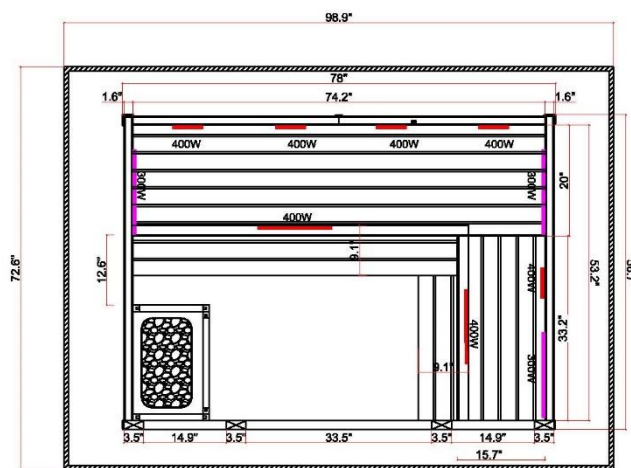
Total power:3700W Vertical Section View
