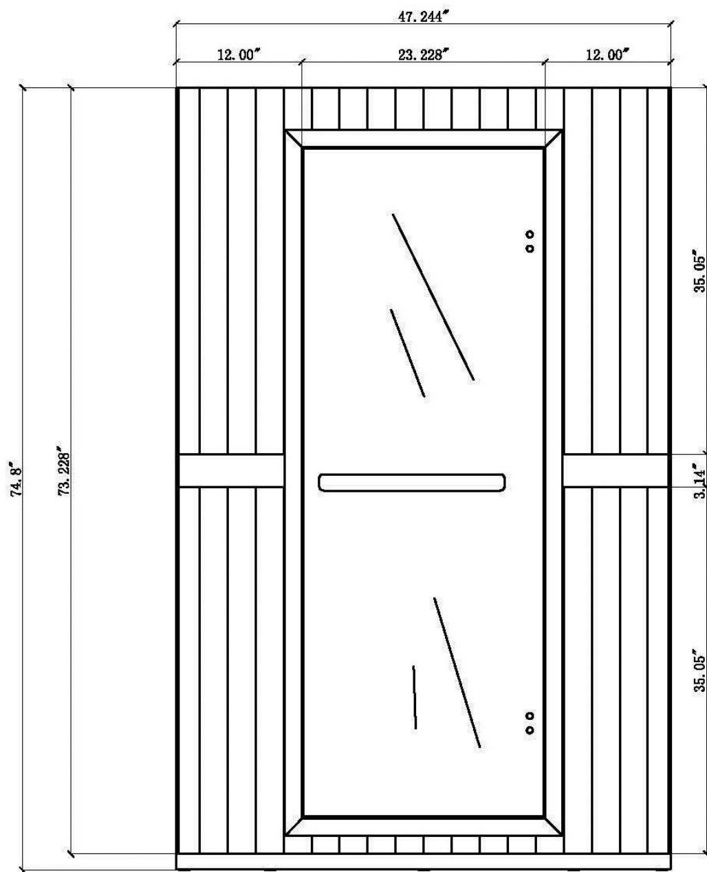
Front View
