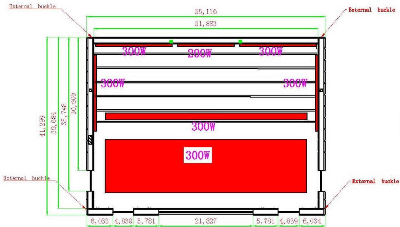
Top View
