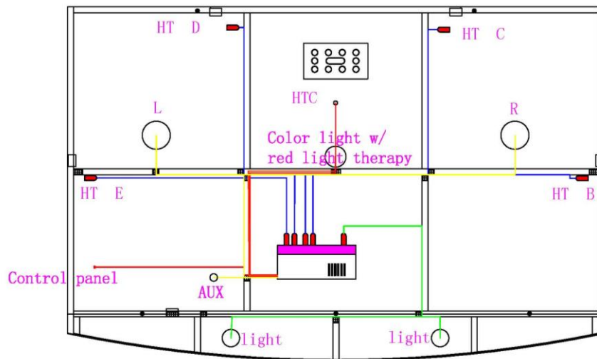
Roof wall panel
