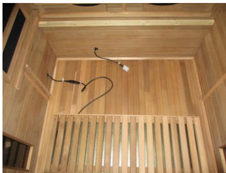
FIG-7 Floor Heater Assembly
