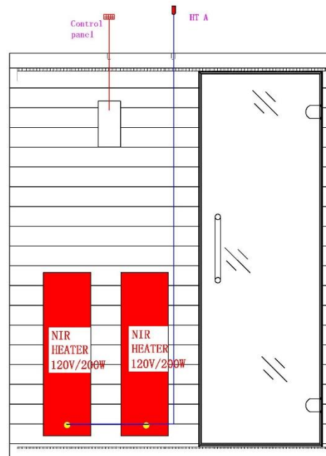
Front wall panel
