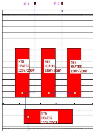
Rear wall panel
