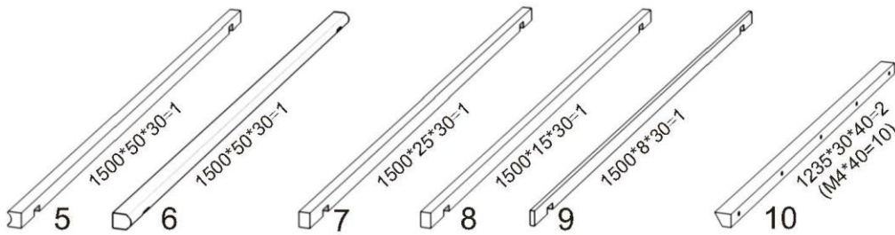
5 2 pcs top filling staves (Width:50mm;50mm) 6 7 3 pcs top filling staves (Width:25mm;15mm;8mm) 8 9 10 Bench back wood plank
