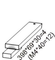
14 Bench support wood
