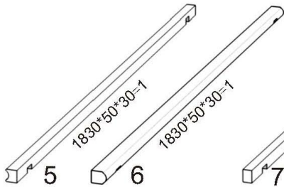
5 2 pcs top filling staves (Width:50mm;50mm)
