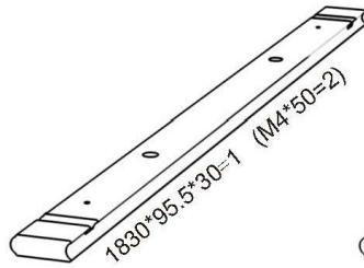
2 The First bottom Stave (with two drain holes and 2 pre-drilled holes)
