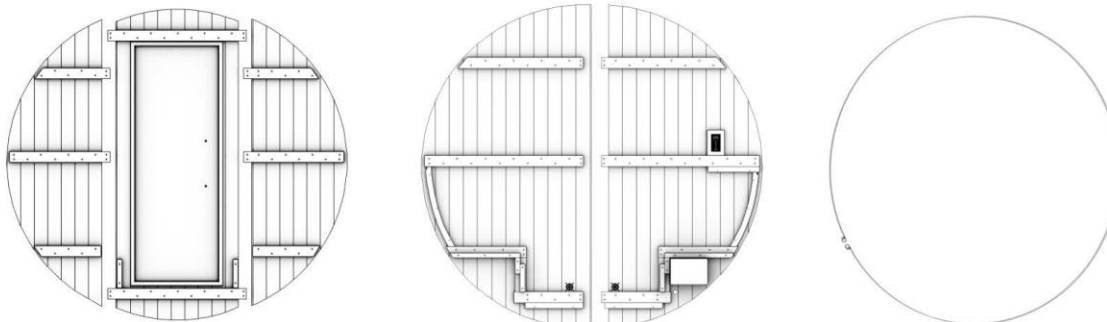
11 2006*791+104*30+20=1 (M4*40=8) 1850.2*615.5+52.2*30+20=2 (M4*40=8) Front wall panel 12 2006*1054.5*30+40=1 2004.1*959.5+42.9*30+40 (M4*40=6) Rear wall panel 13 6352*24*0.5=2 (M195*10=2) Stainless steel band
