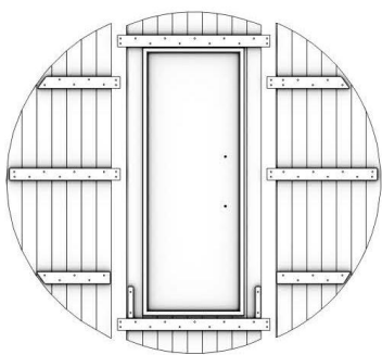
11 2006*791+104*30+20=1 (M4*40=8) 1850.2*615.5+52.2*30+20=2 (M4*40=8) Front wall panel
