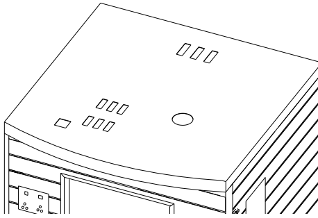
FIG 7 Slip the power cord through Roof Cover (Roof Cover is optional to install)
