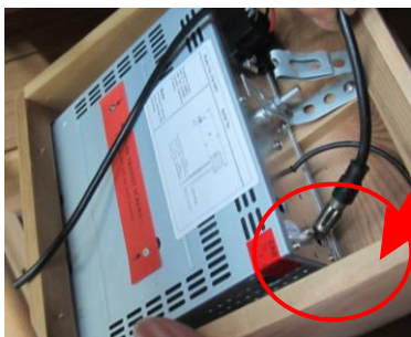
FIG-15 Screw CD Player into sauna room
