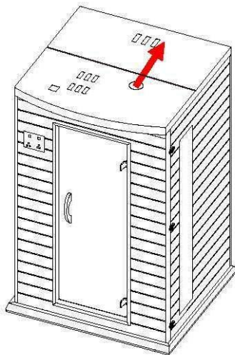
FIG-19 Slip the power cord through Roof Cover Cover
