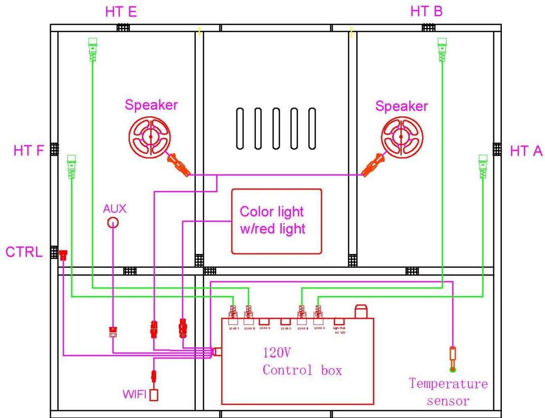
Roof Panel
